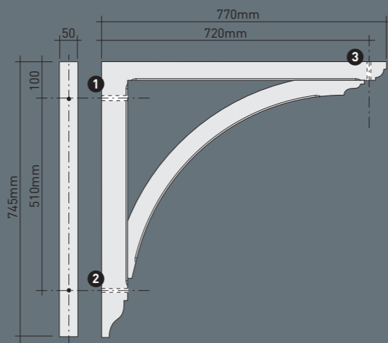
GB04 50 x 745 x 770mm 2" x 29 5 / 16 " x 30 5 / 16 " - structural max. 75kg* - white wood grain finish
